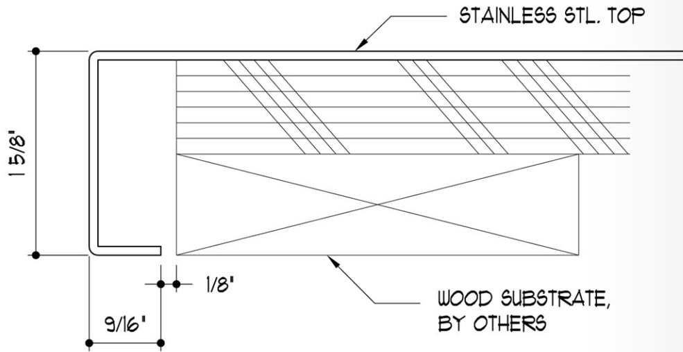
SECTION - WOOD CABINET OPTION
