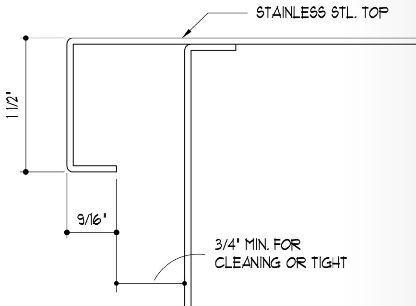
SECTION - METAL CABINET OPTION MEETS N.S.F. REQ'S.
