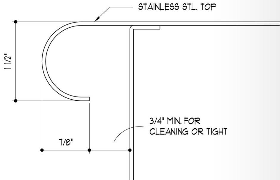
SECTION - METAL CABINET OPTION MEETS N.S.F. REQ'S.
