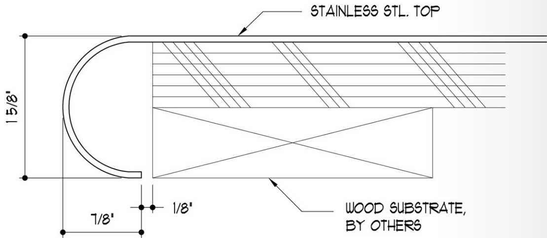
SECTION - WOOD CABINET OPTION
