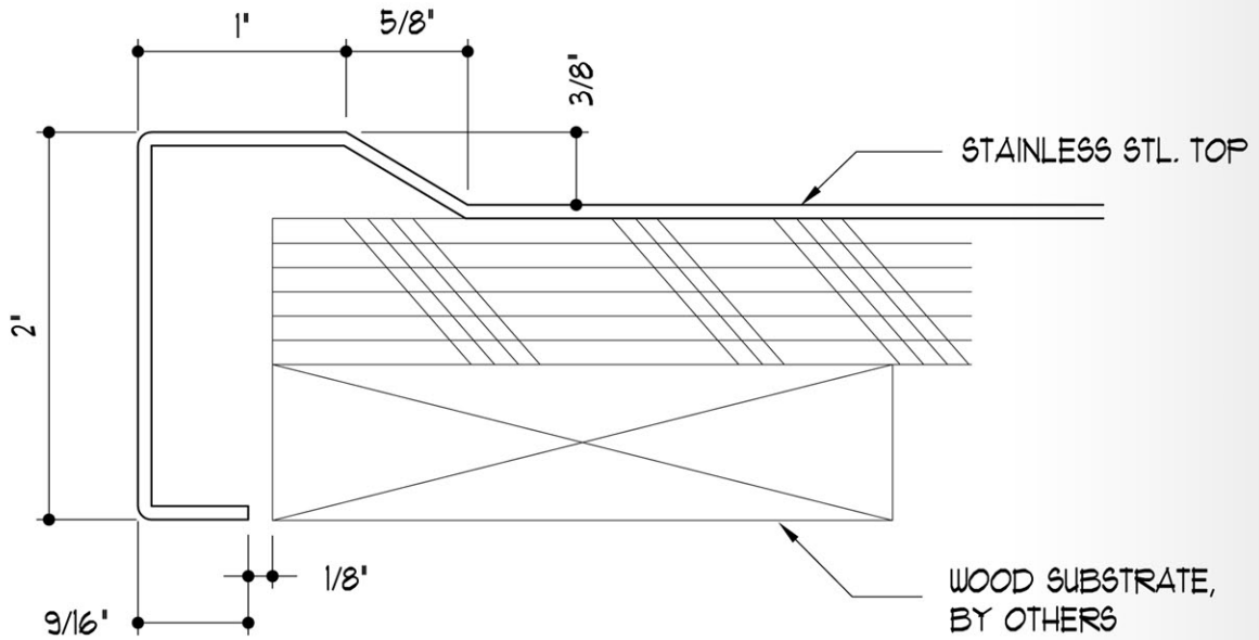
SECTION - WOOD CABINET OPTION
