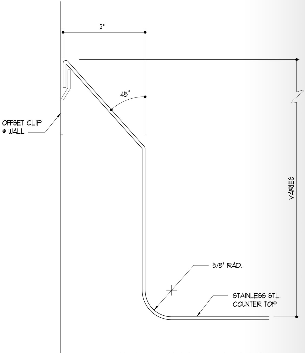
SECTION - DISHTABLE BACKSPLASH
