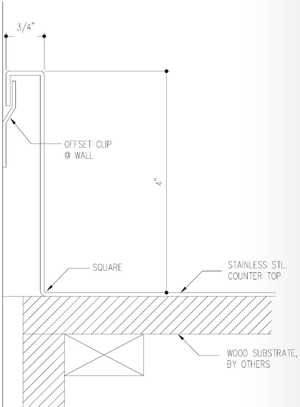
SECTION – COUNTER BACKSPLASH FULL SCALE
